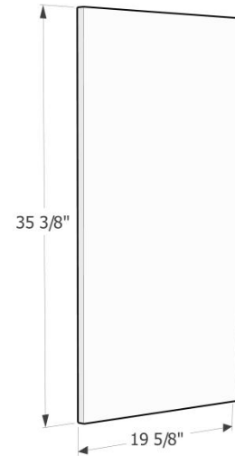
Back View
