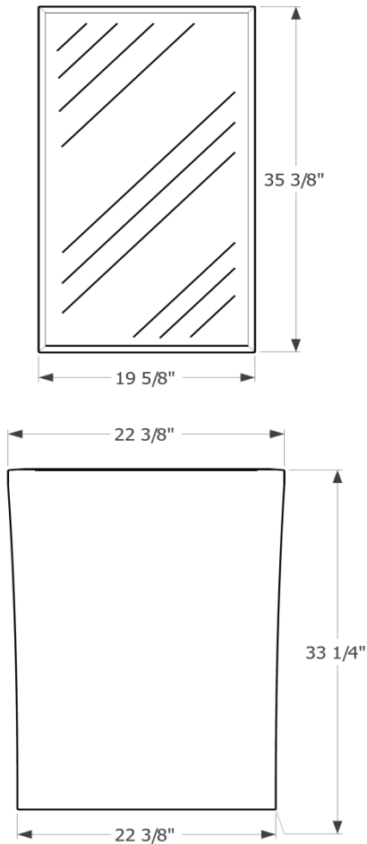
Front View
